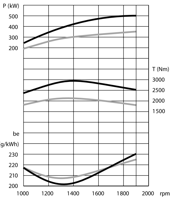
Engines TCD 2015 V6 | TCD 2015 V8
